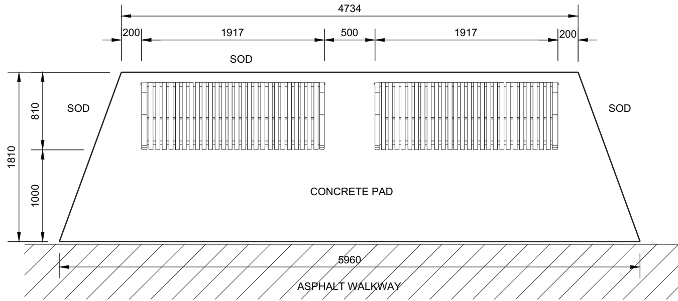
CONCRETE BENCH PAD: PLAN
