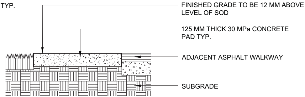
CONCRETE BENCH PAD: SIDE SECTION
